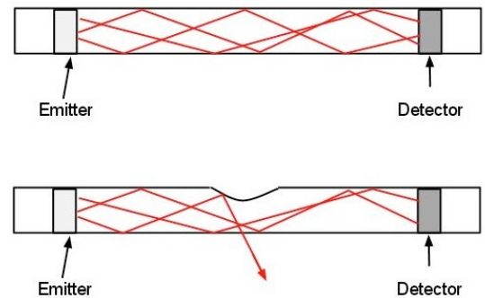
Figure: Top: Cross-section view of the device between an emitter and a detector, in absence of external stimuli. Bottom: Cross-section view of the device showing electromagnetic waves between an emitter and a detector, in presence of an external stimulus deforming the sensing layer
